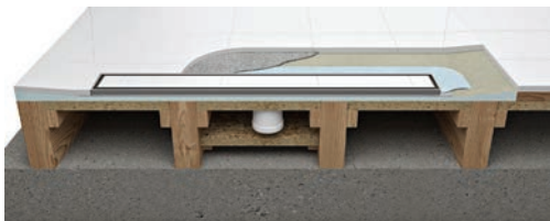
Tray & Drain using underboarding, including under trap
