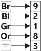
DHW valve V4043H
