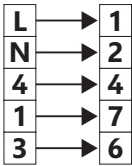
ST 6300 Room stat
