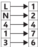
Honeywell CT 6300 Programmer 24 Hr
